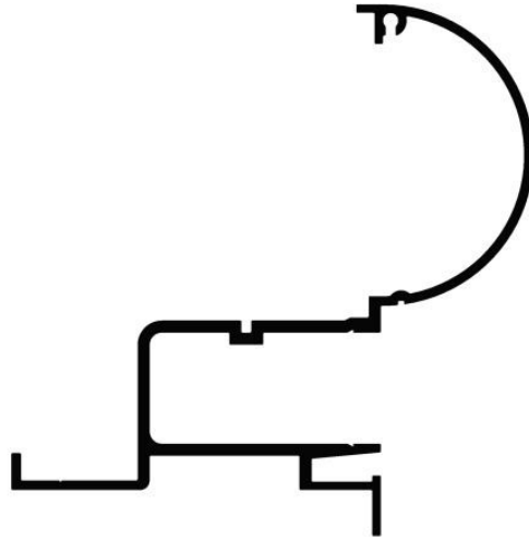
1 - Piece Bullnose
