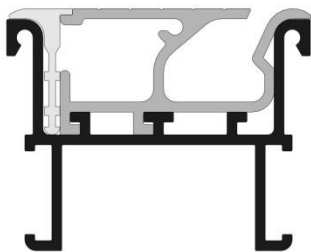
Recessed Horizontal Track
