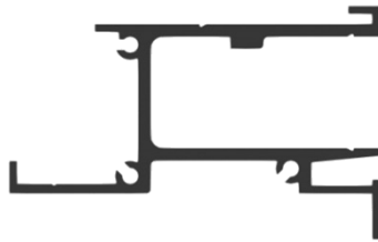
403 Vinyl Liner Encapsulation Retainer
