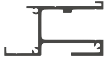
403 Fiberglass Encapsulation Retainer
