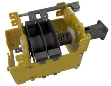
Infinity 4000™ Mechanism
