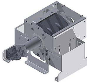
Eclipse Mechanism Deck Mount
