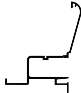
Inclined Coping
