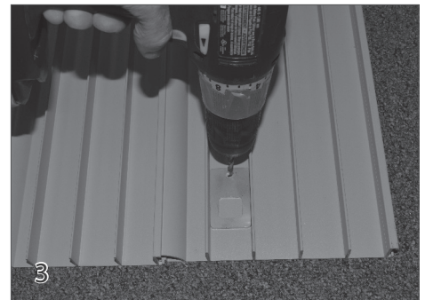
With the backing plate in position, use a drill with a 1/4" drill bit to drill through the small hole in the backing plate and through the lid panel.
