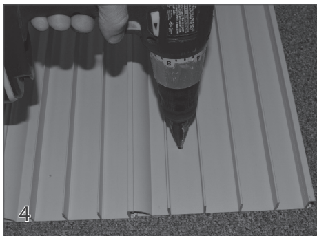
Remove the backing plate. Use the step bit to enlarge the drilled hole from 1/4" to 7/8". Repeat drilling the holes on the other end of the lid.
