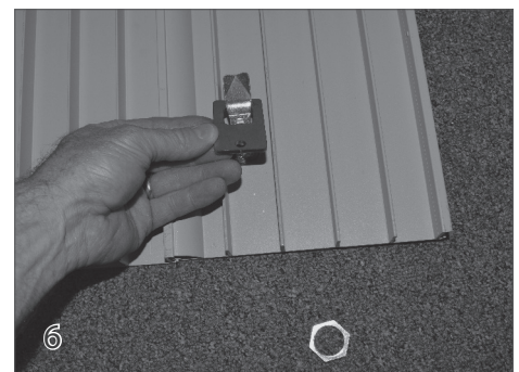
Slide the backing plate over the cam and down around the body of the lock. The backing plate will fit between the ribs of the lid panel.
