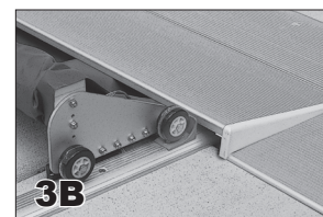
Topguide System
